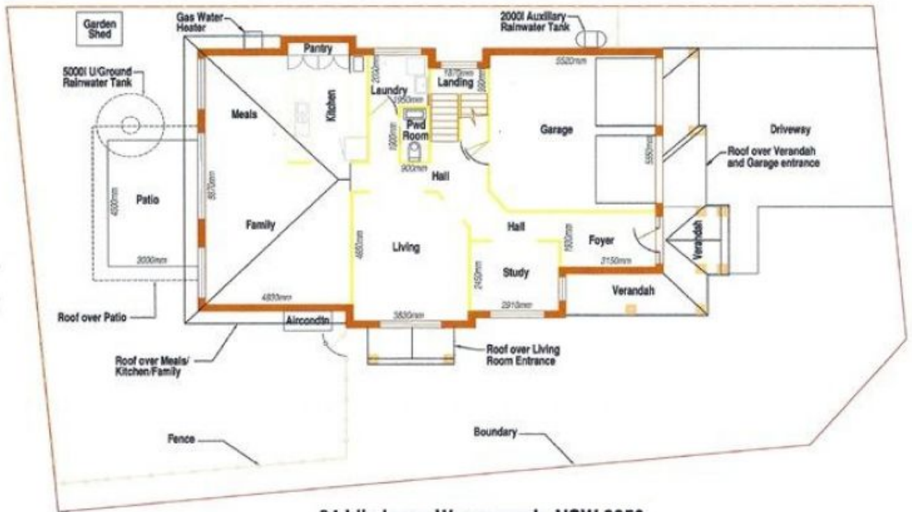
24 Lily Lane, Woongarah, NSW 2259 Allam Ettalong Corner Contemporary GROUND FLOOR PLAN
